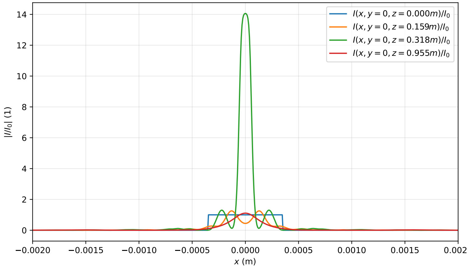
Intensity profile I(x, y = 0, z)/I_0 , \text{Pin}=5.0\text{Pcr} , artificial time
